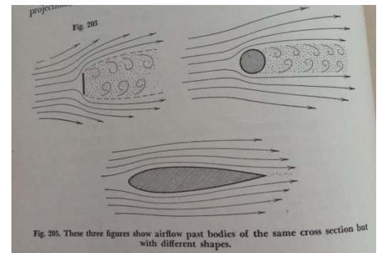
Fig. 205. These three figures show airflow past bodies of the same cross section but with different shapes.
